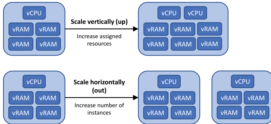
Figure 9.1 You can scale your applications up and down, or in and out. The method you use depends on how your application is built to handle scale. Vertical scale adjusts the resources assigned to a VM or web app, such as the number of CPU cores or amount of memory. This method to scale an application works well if the application runs only one instance. Horizontal scale changes the number of instances that run your application and helps increase availability and resiliency.
