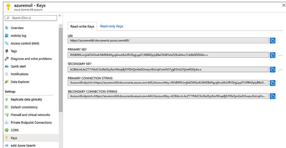
Figure 10.11 The Keys section of your Cosmos DB account lists the connection information and access keys. You need this information when you build and run applications, such as in the end-of-chapter lab.
