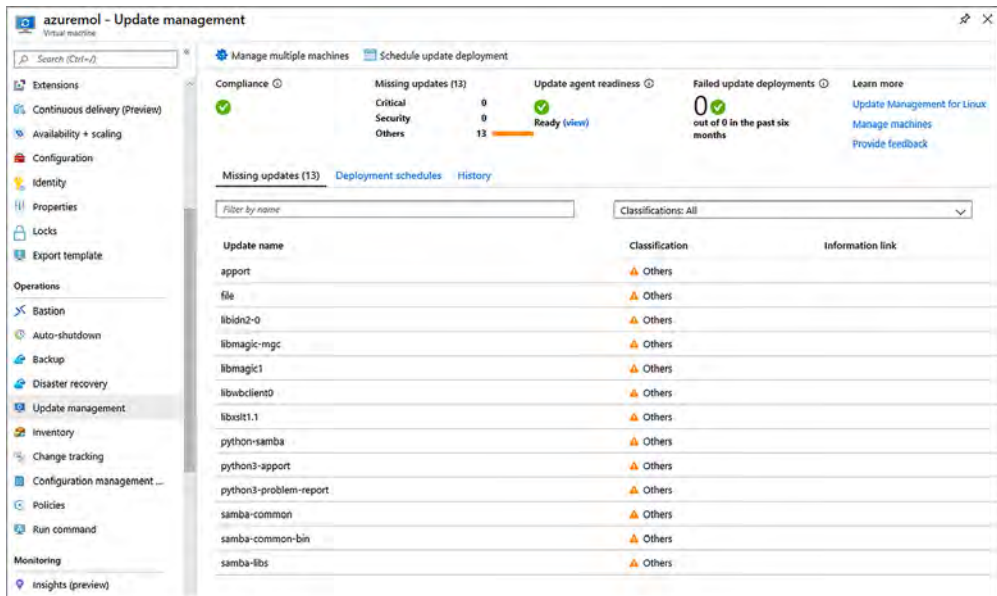
Figure 16.10 When the VM agent has scanned for compliance, a list of available updates is provided. Depending on the OS and version, Update Management may be able to work with the Log Analytics workspace and Azure Monitor to classify the updates based on severity or to provide links to the relevant update hotfix pages.
