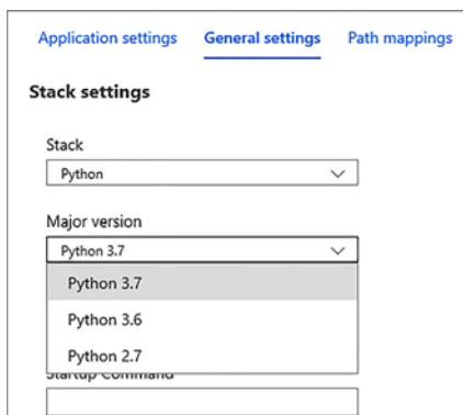
Figure 3.2 Select a specific version of a language in the Web Apps application settings.
