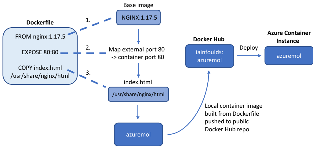
Figure 19.6 A Dockerfile was used to build a complete container image: azuremol. This image was pushed to an online public registry called Docker Hub. Now you can create a container instance using this prebuilt public image from Docker Hub, which provides a ready-to-run application image.
